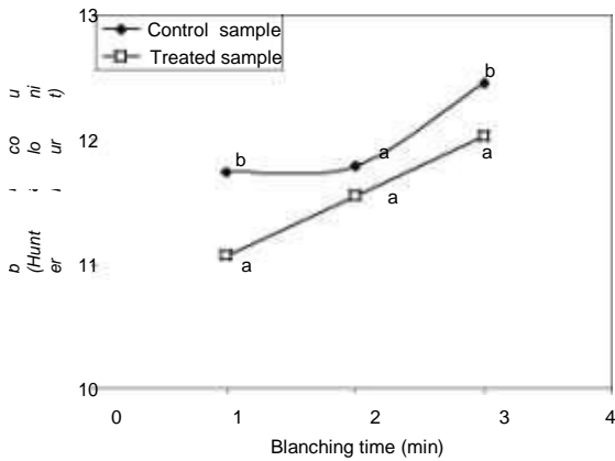
Figure 3. b-value colour parameter of tomato puree samples. Different letters corresponds to the samples of a particular blanching time differ significantly ( P < 0.05 ).
